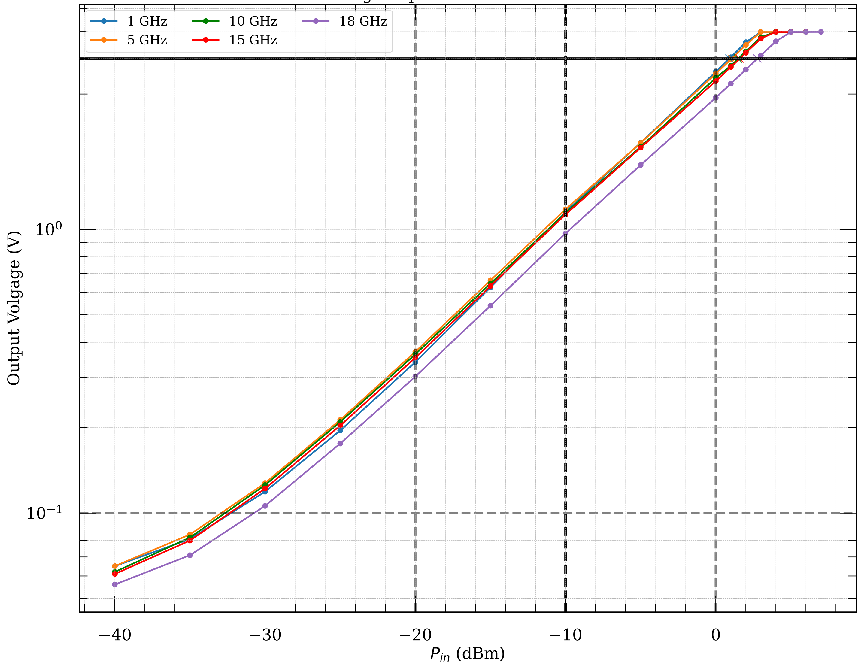
Measured voltage-to-power curve of detector module075
